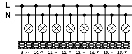
f Connection of the loads (device EK-FG1-TP used as 8-fold binary output)
