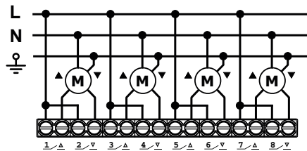
f Connection of the loads (device EK-FG1-TP used as 8-fold binary output)
