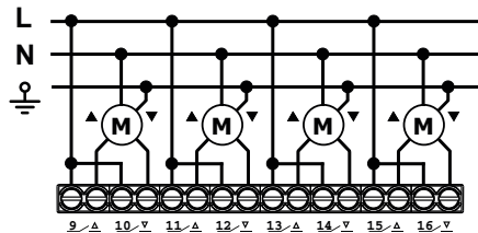
g Connection of the loads (device EK-FG1-TP used as 4-fold blind actuator)
