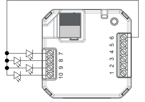
Connection of outputs (low-consumption LEDs)
